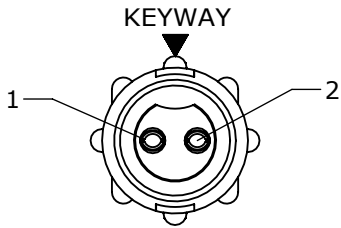
FACE VIEW 18282-2SG-3XX
