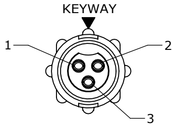
FACE VIEW 18282-3SG-3XX
