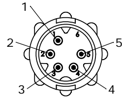
FACE VIEW 18982-5PG-5XX 5 POSITION A-KEY
