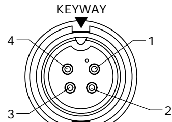
FACE VIEW ASSY: 3282-4PG-5XX
