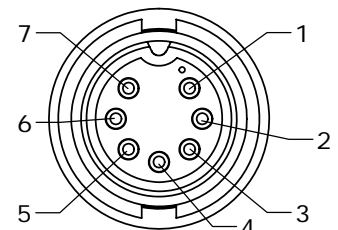
FACE VIEW ASSY: 3282-7PG-5XX
