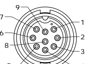
FACE VIEW ASSY: 3282-9PG-5XX
