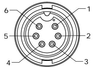
FACE VIEW ASSY: 3282-6PG-5XX
