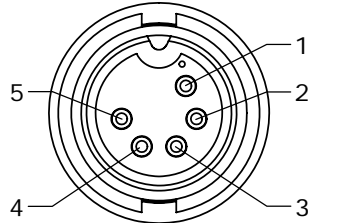
FACE VIEW ASSY: 3282-5PG-5XX
