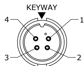
FACE VIEW P/N: 3282-4SG-5XX
