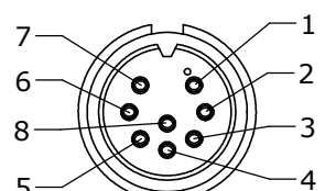
FACE VIEW P/N: 3282-8SG-5XX
