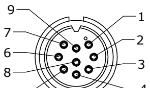
FACE VIEW P/N: 3282-9SG-5XX
