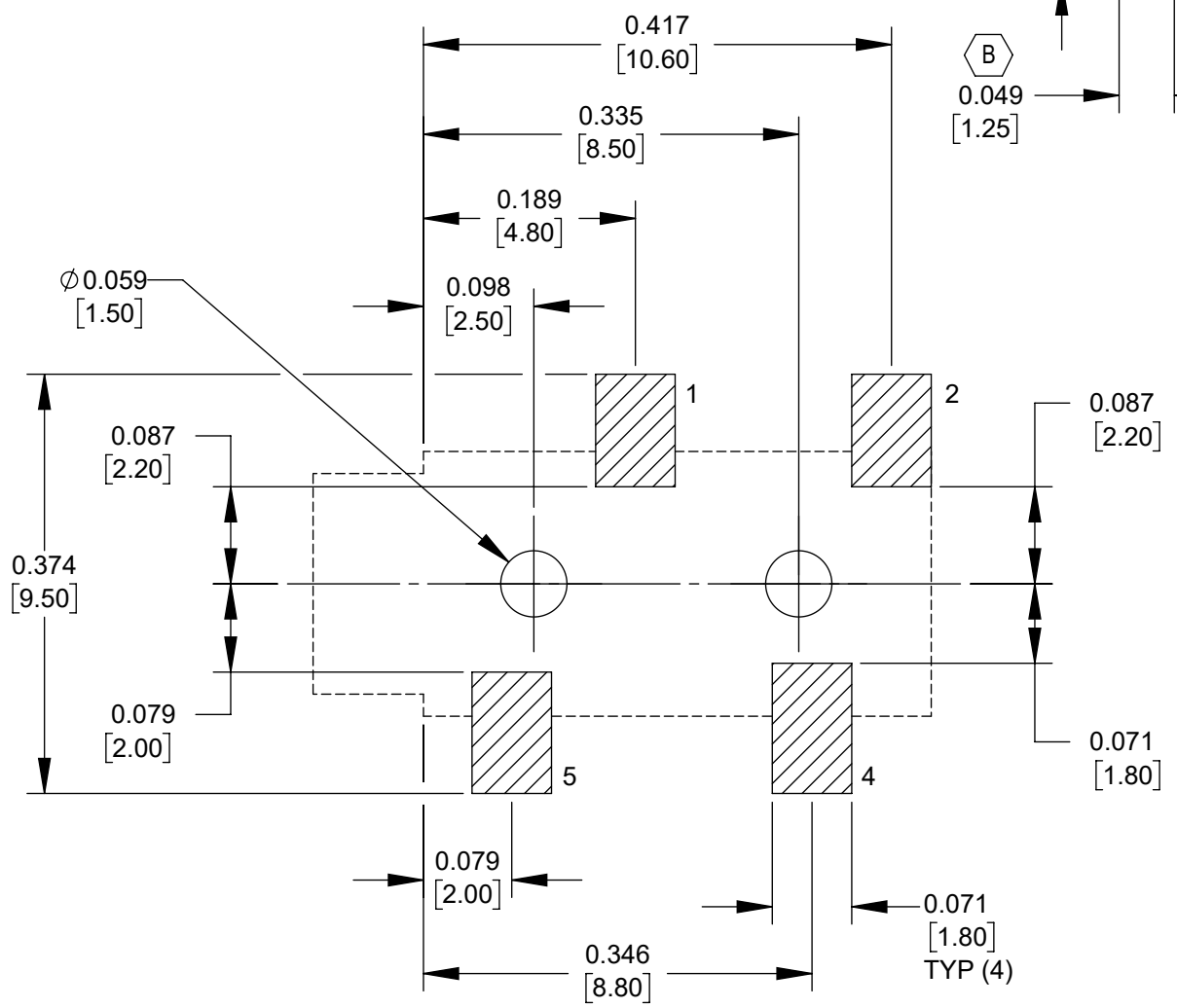
PCB LAYOUT (B) COMPONENT SIDE TOLERANCE: ±0.002 [±0.05]
