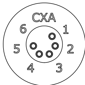
WIRING VIEW ASSY: 4280-5SG-300
