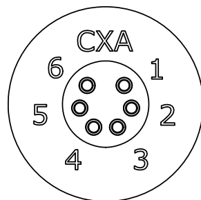
WIRING VIEW ASSY: 4280-6SG-300
