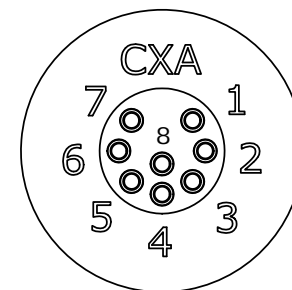
WIRING VIEW ASSY: 4280-8SG-300
