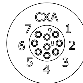
WIRING VIEW ASSY: 4280-9SG-300
