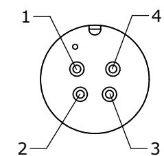
MATING FACE 4282-4PG-300
