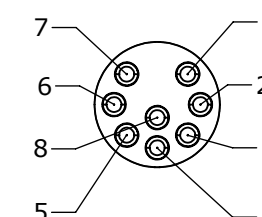
WIRING VIEW 4282-8PG-300
