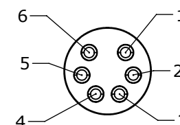
WIRING VIEW 4282-6PG-300
