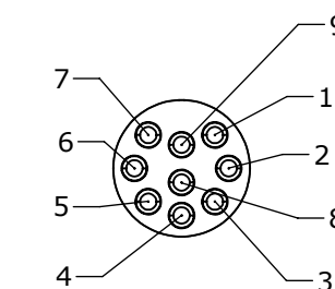
WIRING VIEW 4282-9PG-300
