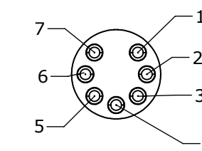
WIRING VIEW 4282-7PG-300
