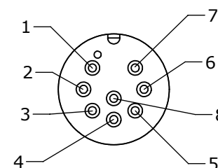
MATING FACE 4282-8PG-300
