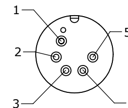
MATING FACE 4282-5PG-300
