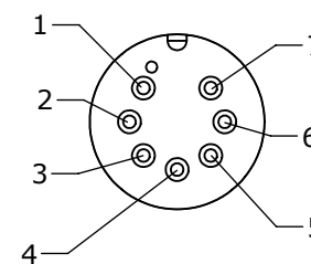
MATING FACE 4282-7PG-300
