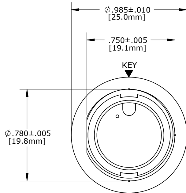
FACE VIEW
