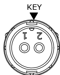
FACE VIEW 5182-2PG-5XX
