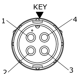
FACE VIEW 5182-4PG-5XX
