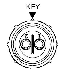
WIRE VIEW 5182-2PG-5XX
