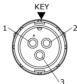
FACE VIEW 5182-3PG-5XX
