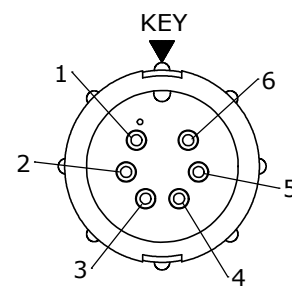
FACE VIEW 5282-6PG-5XX
