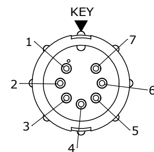
FACE VIEW 5282-7PG-5XX
