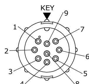
FACE VIEW 5282-9PG-5XX
