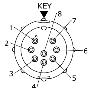
FACE VIEW 5282-8PG-5XX
