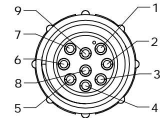
WIRE VIEW 5282-9SG-3XX SHOWN
