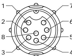
FACE VIEW ASSY: 5282-8SG-3XX
