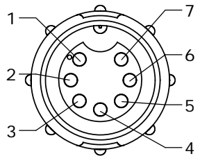
FACE VIEW 5282-7SG-3XX
