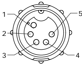
FACE VIEW ASSY: 5282-5SG-3XX
