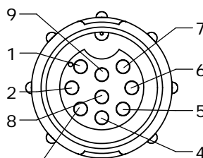
FACE VIEW ASSY: 5282-9SG-3XX
