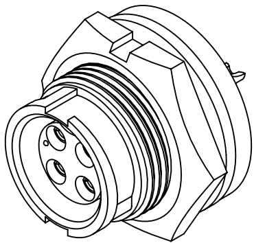
ASSEMBLED VIEW FOR CUSTOMER REFERENCE ONLY 7382-4SG-300 SHOWN
