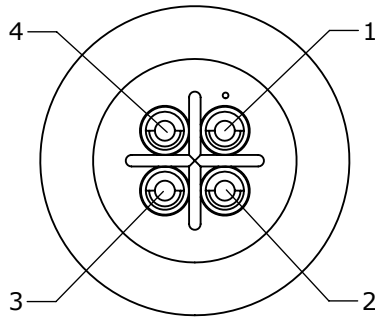
WIRING VIEW 7382-4SG-300
