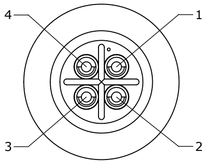
WIRING VIEW 7382-4SG-3ES
