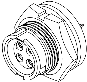
ASSEMBLED VIEW FOR CUSTOMER REFERENCE ONLY 7382-4SG-3ES SHOWN
