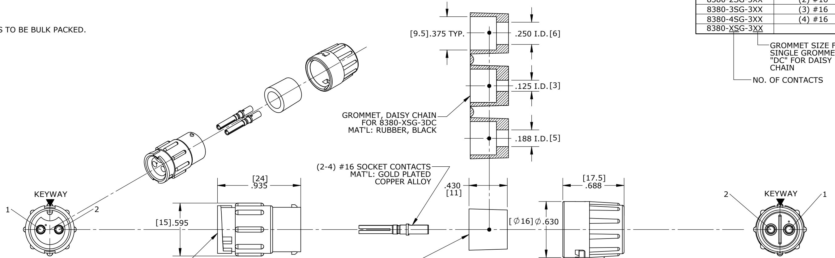
FACE VIEW 8380-2SG-3XX
