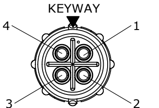
WIRE VIEW 8380-4SG-3XX
