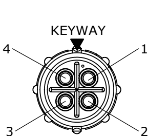
WIRE VIEW 8380-4SG-3XX
