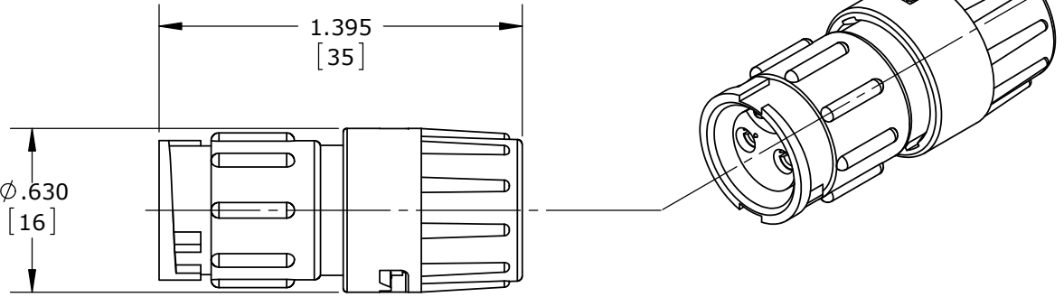
ASSEMBLED VIEWS FOR CUSTOMER REF. 8380-2SG-3XX SHOWN
