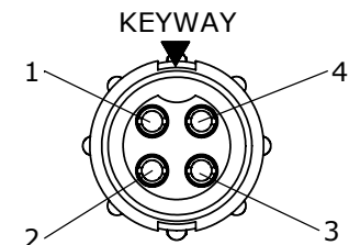
FACE VIEW 8380-4SG-3XX
