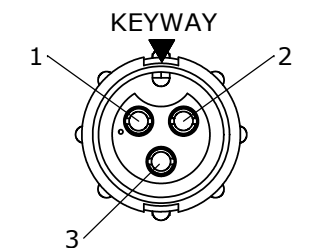
FACE VIEW 8380-3SG-3XX
