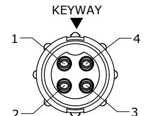
FACE VIEW 8382-4SG-5XX
