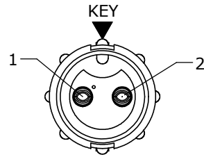
FACE VIEW 8382-2SG-5XX
