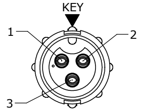
FACE VIEW 8382-3SG-5XX
