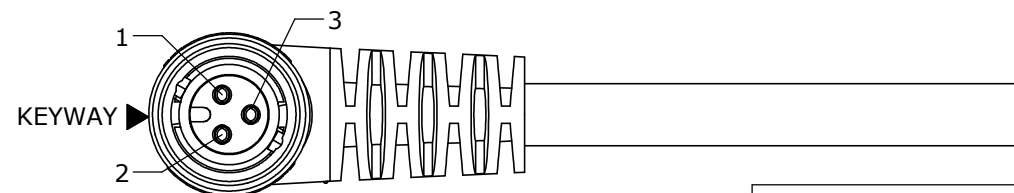
FACE VIEW P/N: CARA162803SXXX90
