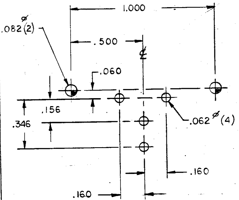
.062 P.C. BOARD, COMPONENT SIDE.
