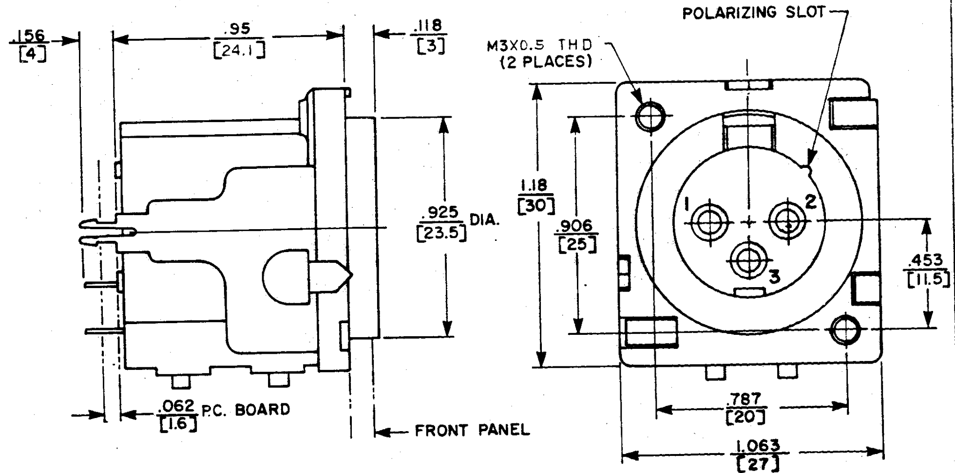
.062 P.C. BOARD, COMPONENT SIDE.
