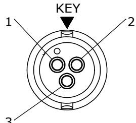
WIRING VIEW W16280-3PG-P-5XX
