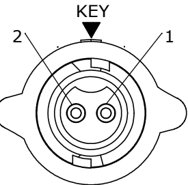
FACE VIEW W16280-2PG-P-5XX
