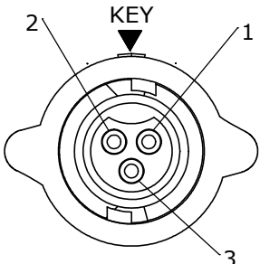
FACE VIEW W16280-3PG-P-5XX
