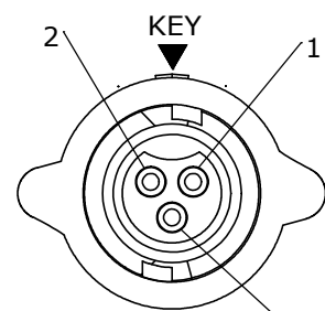
FACE VIEW W16282-3PG-P-5XX
