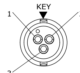
WIRING VIEW W16282-3PG-P-5XX
