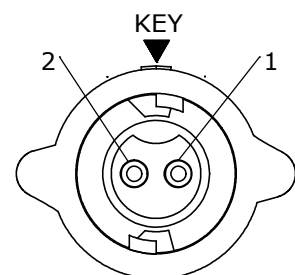
FACE VIEW W16282-2PG-P-5XX
