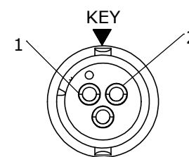
WIRING VIEW W16282-2PG-P-5XX
