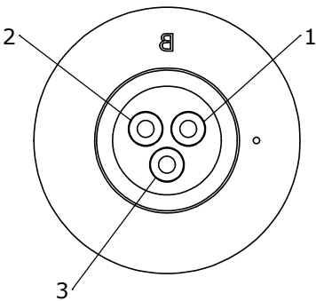
WIRE VIEW W17281-3SG-P-300
