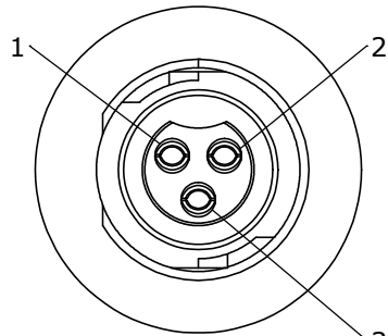
FACE VIEW W17281-3SG-P-300
