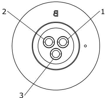
WIRE VIEW W17282-3SG-P-300
