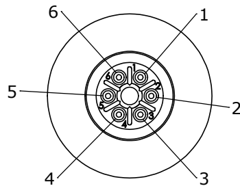
WIRE VIEW W17984-6SG-P-3ES
