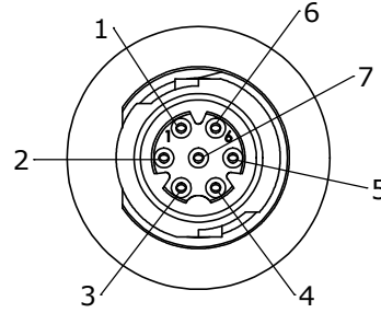
FACE VIEW W17984-7SG-P-3ES 7 POSITION A-KEY
