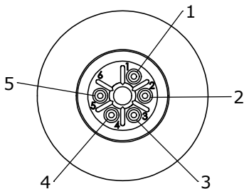
WIRE VIEW W17984-5SG-P-3ES
