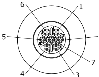
WIRE VIEW W17984-7SG-P-3ES
