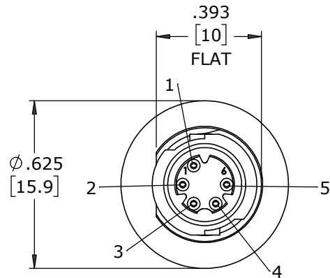
FACE VIEW W17984-5SG-P-3ES 5 POSITION A-KEY
