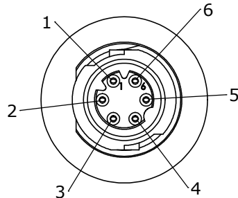
FACE VIEW W17984-6SG-P-3ES 6 POSITION B-KEY
