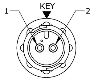
FACE VIEW W18282-2PG-P-5XX
