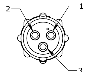
WIRING VIEW W18282-3PG-P-5XX
