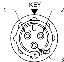
FACE VIEW W18282-3PG-P-5XX
