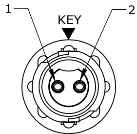
FACE VIEW W18282-2SG-P-5XX
