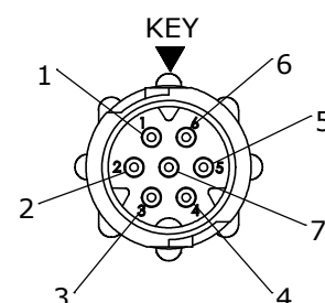
FACE VIEW W18980-7PG-P-5XX A-KEY
