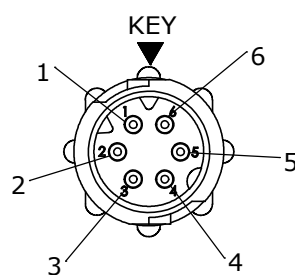
FACE VIEW W18980-6PG-P-5XX B-KEY
