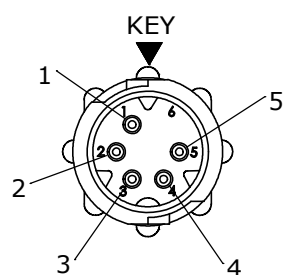
FACE VIEW W18980-5PG-P-5XX A-KEY
