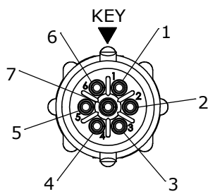
WIRING VIEW W18980-7PG-P-5XX
