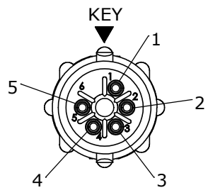
WIRING VIEW W18980-5PG-P-5XX
