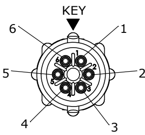
WIRING VIEW W18980-6PG-P-5XX
