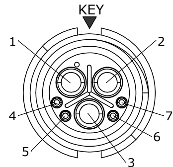
WIRE VIEW
