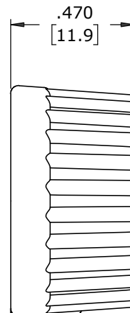
COUPLING RING, STD MAT'L: UV PBT, BLACK
