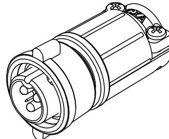
WINGED COUPLING RING P/N: W3B82-7PG-5XXW
