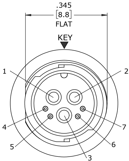
FACE VIEW
