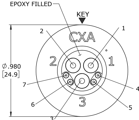
WIRE VIEW
