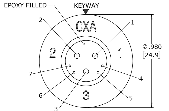
WIRE VIEW
