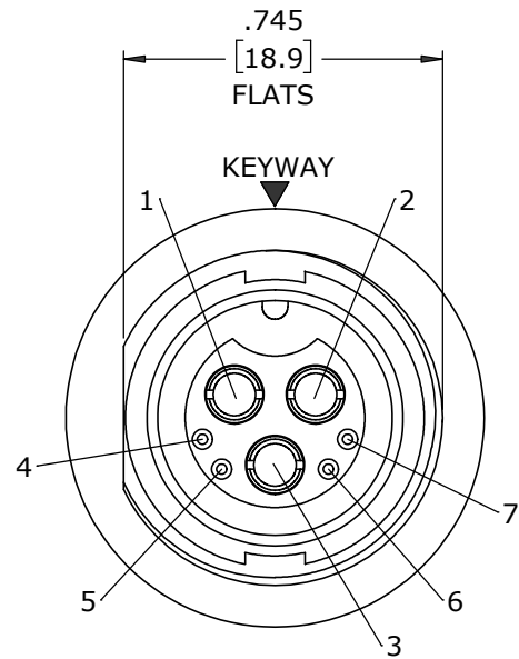
FACE VIEW
