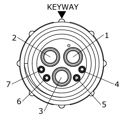
WIRE VIEW
