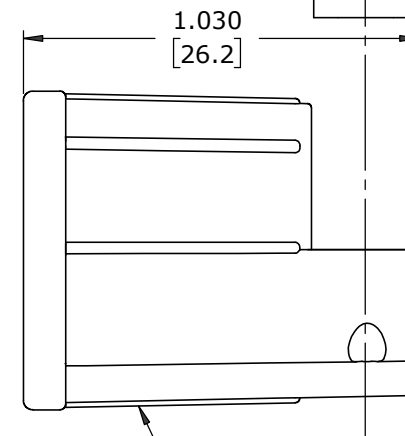
BACKSHELL MAT'L: UV PBT, BLACK
