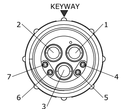
WIRE VIEW
