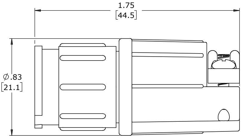
ASSEMBLED VIEW FOR CUSTOMER REF ONLY
