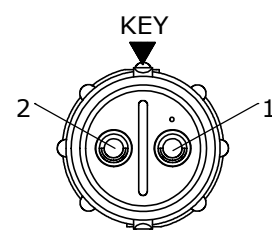
WIRE VIEW W8382-2PG-P-5XX
