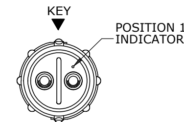
WIRING END W8382-2PG-P-5XX SHOWN WITHOUT HARDWARE
