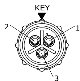
WIRE VIEW W8382-3PG-P-5XX
