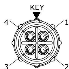
WIRE VIEW W8382-4PG-P-5XX
