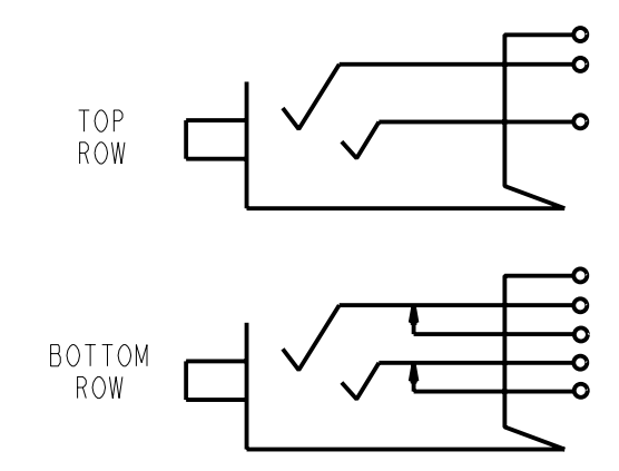
IT JACK SCHEMATIC
