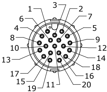
FACE VIEW 15280-20PG-4XX
