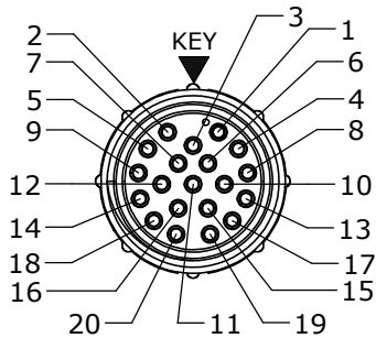
WIRE VIEW 15280-20PG-4XX
