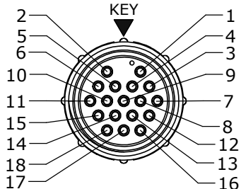
WIRE VIEW 15280-18PG-4XX
