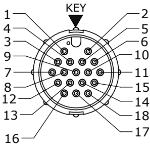
FACE VIEW 15280-18PG-4XX
