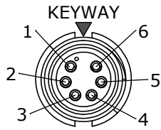
WIRE VIEW 3282-6SG-4XXW
