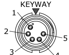
WIRE VIEW 3282-5SG-4XXW
