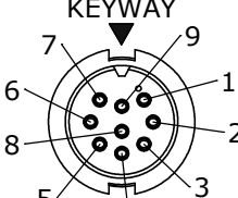
FACE VIEW 3282-9SG-4XXW
