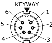
FACE VIEW 3282-6SG-4XXW
