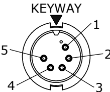
FACE VIEW 3282-5SG-4XXW
