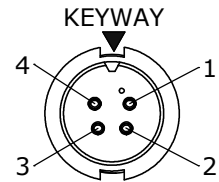
FACE VIEW 3282-4SG-4XXW
