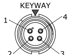
WIRE VIEW 3282-4SG-4XXW
