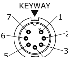
FACE VIEW 3282-7SG-4XXW
