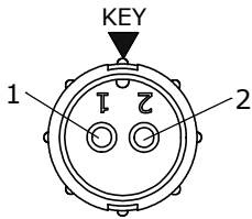
FACE VIEW 5182-2PG-4XX
