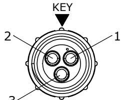
WIRE VIEW 5182-3PG-4XX
