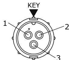
FACE VIEW 5182-3PG-4XX
