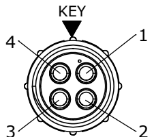
WIRE VIEW 5182-4PG-4XX
