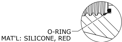
DETAIL A
