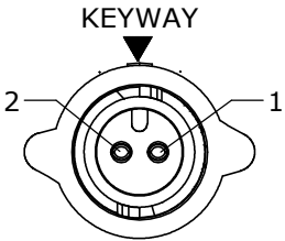
END "A"
