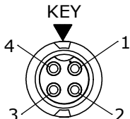
END "A" FACE VIEW CARA63804PPXXX90
