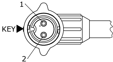
END "A" FACE VIEW CARA63802PPXXX90 SHOWN
