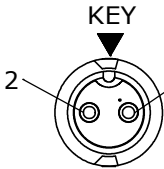
END "A" FACE VIEW CARA63802PPXXX90
