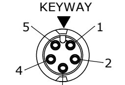
END "A" FACE VIEW CARA63805SPXXX90
