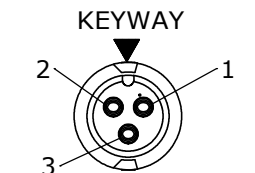
END "A" FACE VIEW CARA63803SPXXX90
