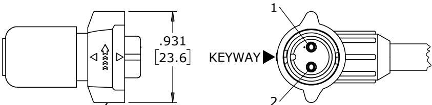
END "A" FACE VIEW CARA63802SPXXX90 SHOWN
