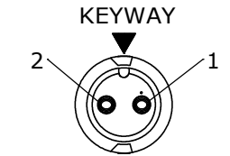
END "A" FACE VIEW CARA63802SPXXX90
