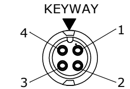
END "A" FACE VIEW CARA63804SPXXX90
