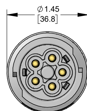
EP7L5M10CG 5-POLE MALE
