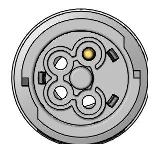
EP7L4M10BG 4-POLE MALE
