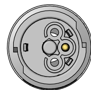
EP7L3M10AG 3-POLE MALE
