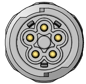
EP7P5M10G 5-POLE FEMALE
