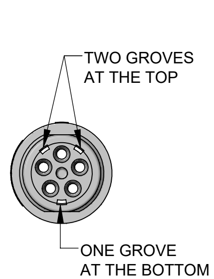
FIG B: SHELL ASSEMBLY REAR VIEW
