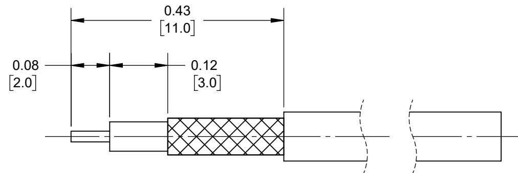
RECOMMENDED RG-316/U CABLE STRIP DIMENSIONS (CUSTOMER SUPPLIED CABLE)
