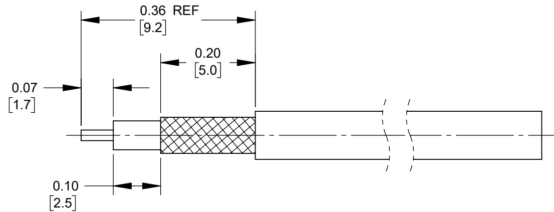
RECOMMENDED RG-316/U CABLE STRIP DIMENSIONS
