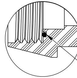
O-RING #2 MAT'L: SILICONE, RED
