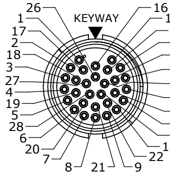
WIRE FACE
