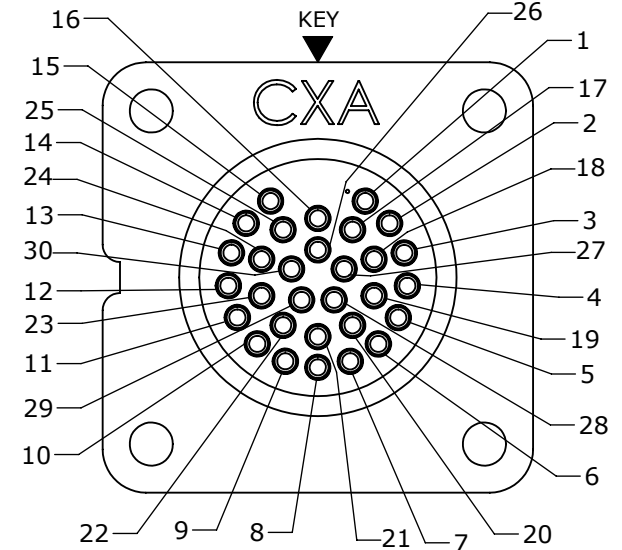
WIRE VIEW
