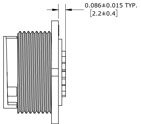
CONTACT HEIGHT FOR CUSTOMER REFERENCE
