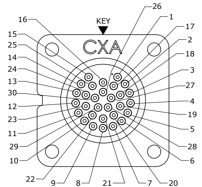
WIRE VIEW
