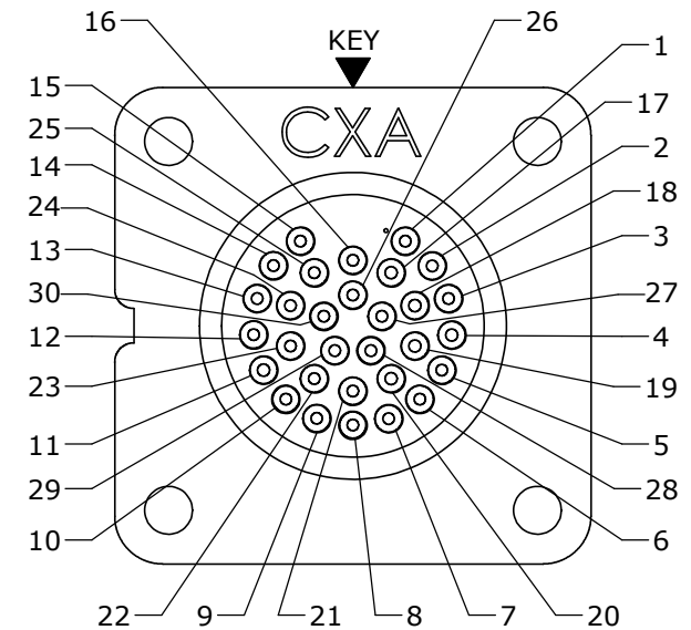
WIRE VIEW
